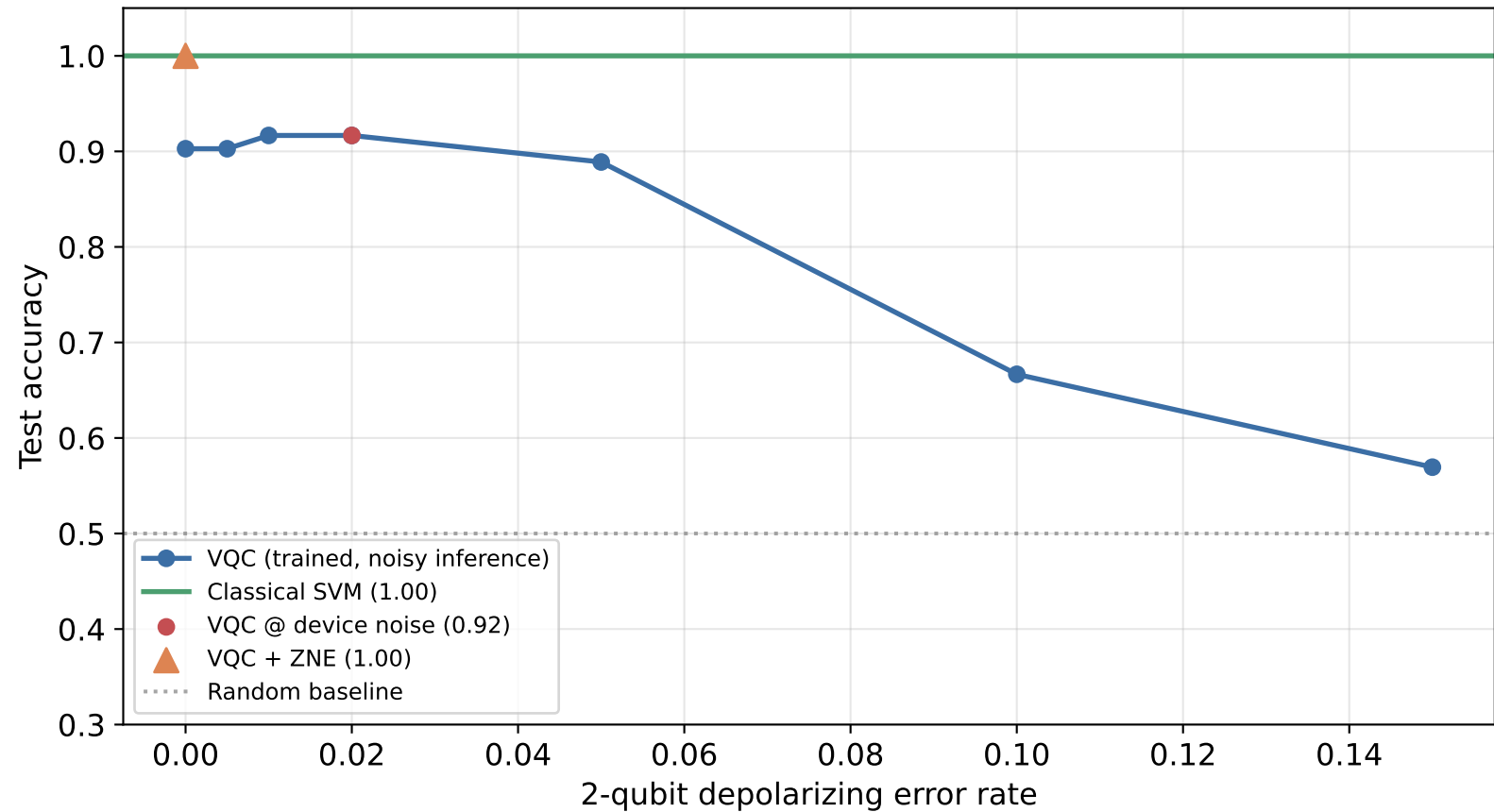
Noise Resilience of the Trained VQC
