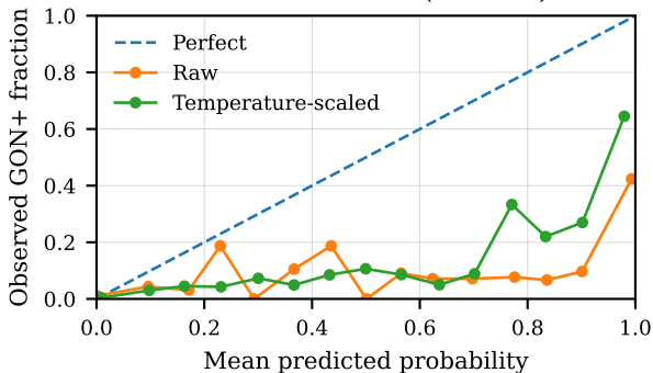
OIA-ODIR-TRAIN (n=3129)
