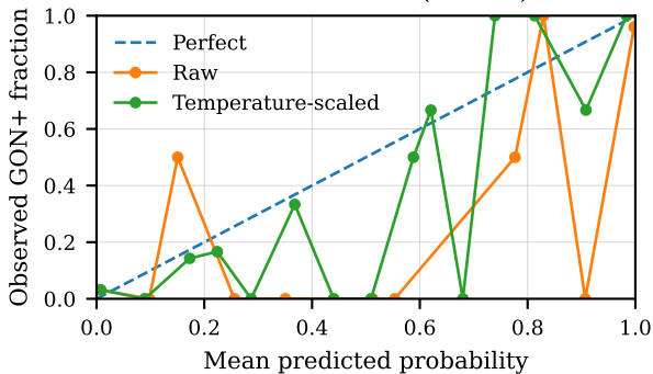
REFUGE1-train (n=400)
