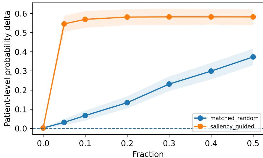
ConvNeXtTiny — deletion
