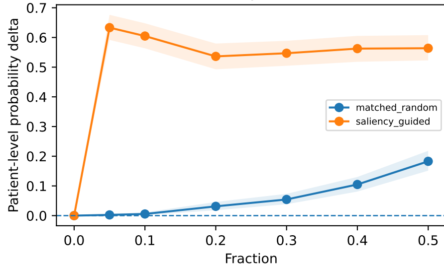
ConvNeXtTiny — insertion
