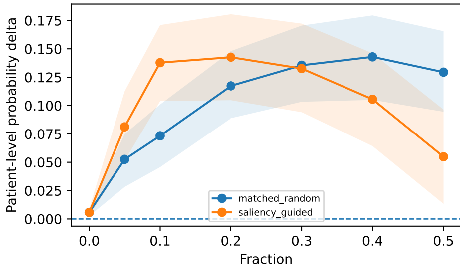
ConvNeXtTiny — deletion
