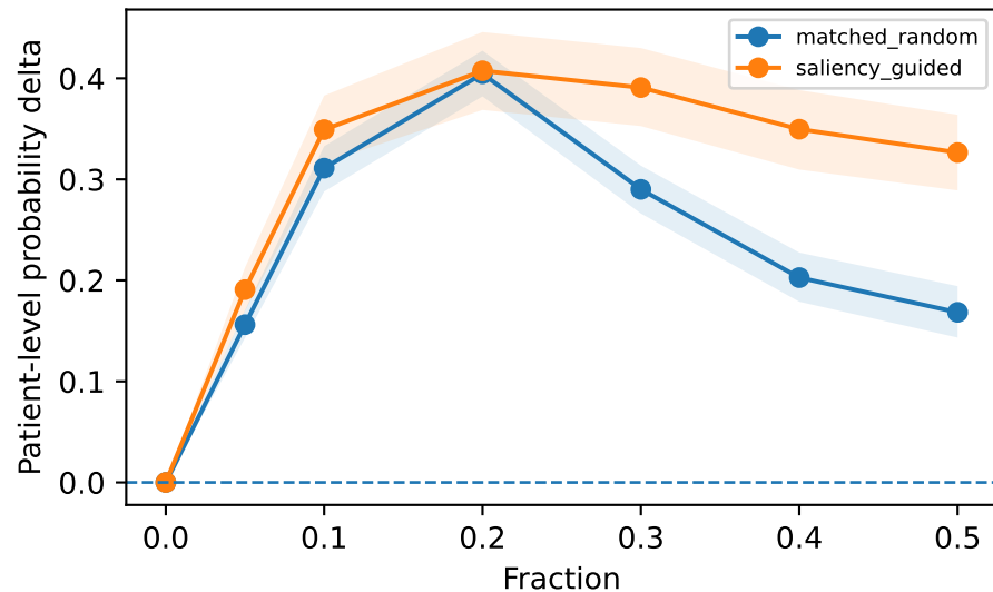
ConvNeXtTiny — insertion
