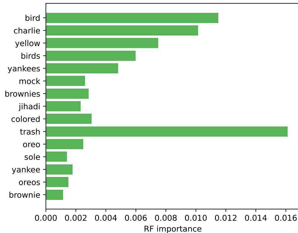
Top 15 Features Neither (2)
