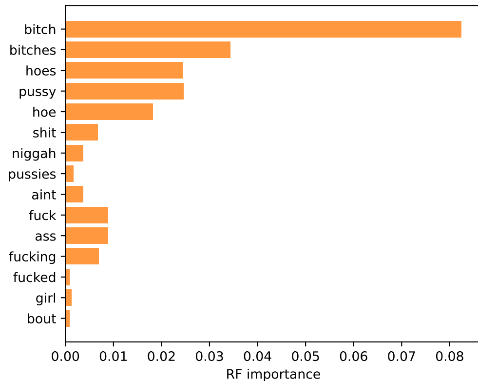
Top 15 Features Offensive (1)
