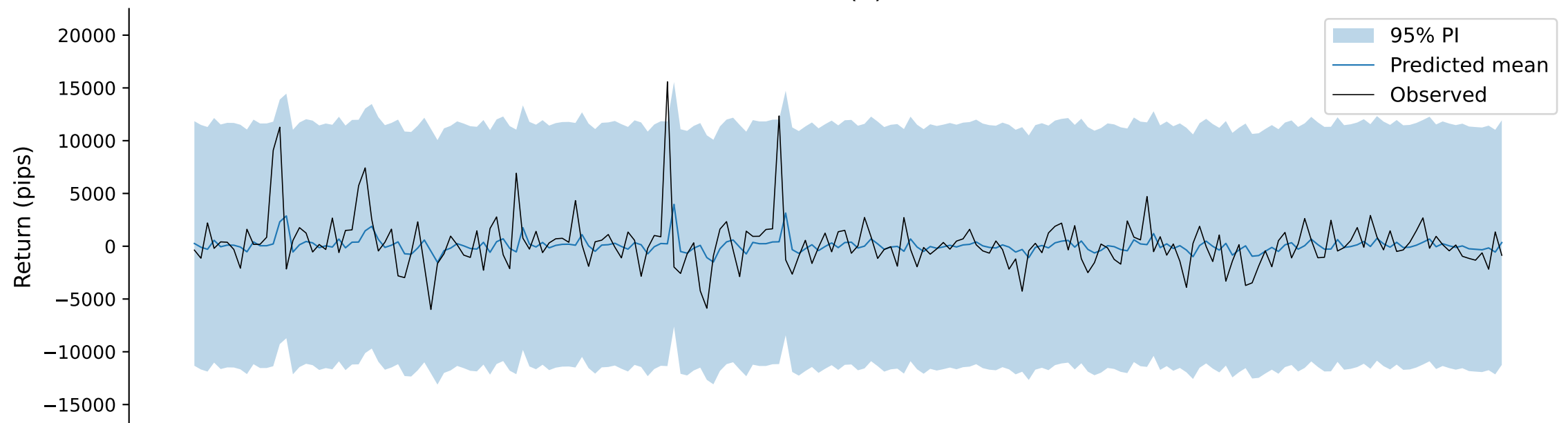
Prediction intervals — XAUUSD (k = 10 ticks)
