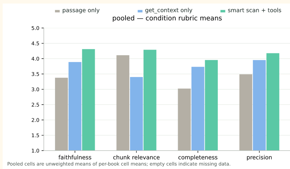
Figure 1: Mean-pooled scores (across all three books)
