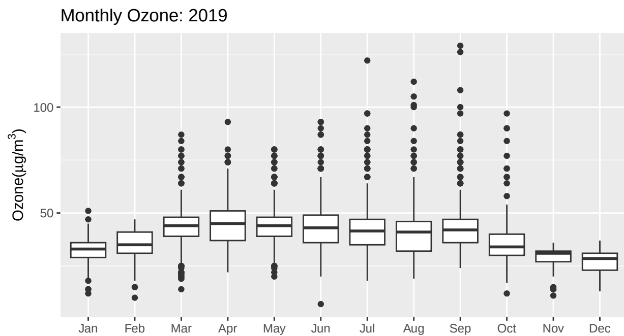
Figure 2: Monthly Ozone (2019)
