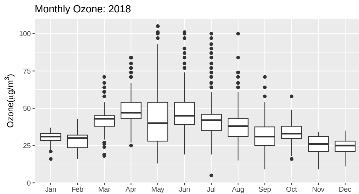
Figure 1: Monthly Ozone (2018)
