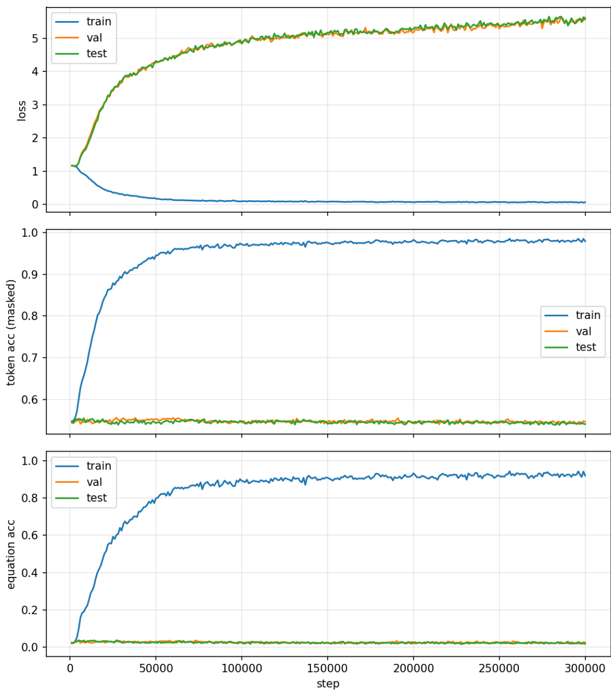
Figure 4: Part 1.4 low weight decay ablation: division mod 97, \text{weight\_decay} = 0.1 , 300k steps.
