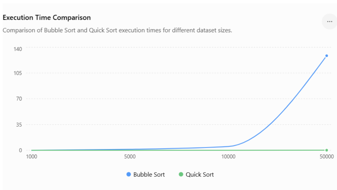
Figure D.1: Comparison of execution times between Bubble Sort and Quick Sort. Bubble Sort exhibits a dramatic increase in execution time as dataset size increases, while Quick Sort maintains low execution times.
