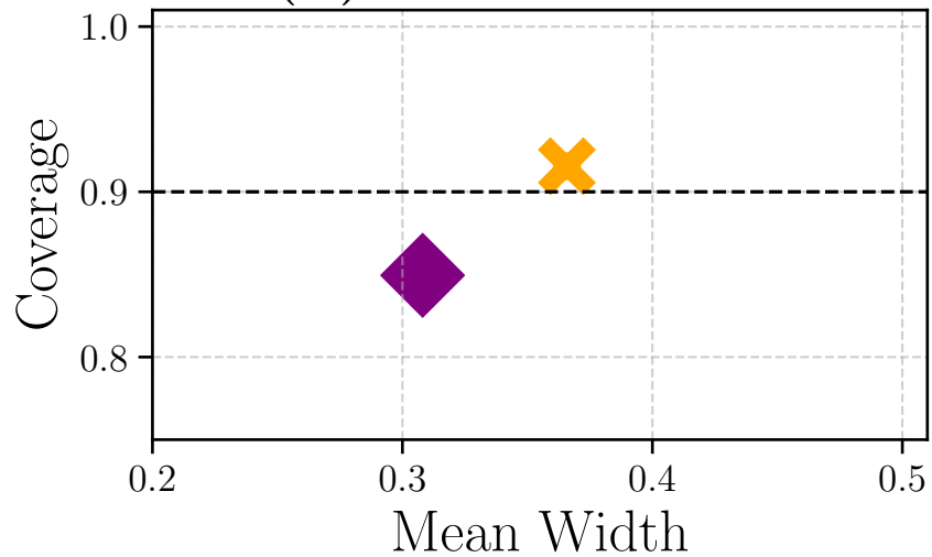
(B) Income: > $70K
