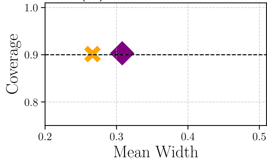
(A) Income: \leq $70K
