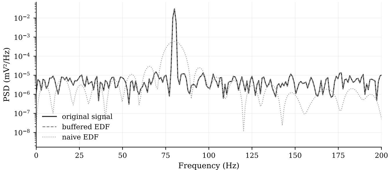
Spectral contamination caused by silent padding
