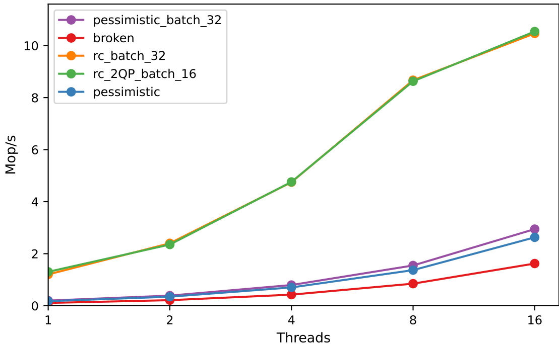
Threads vs Throughput for sm110p with 1024 size
