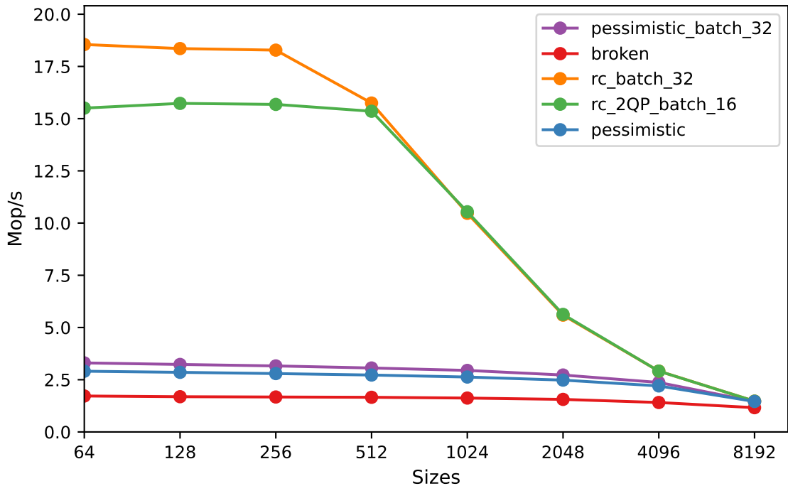
Sizes vs Throughput for sm110p with 16 threads
