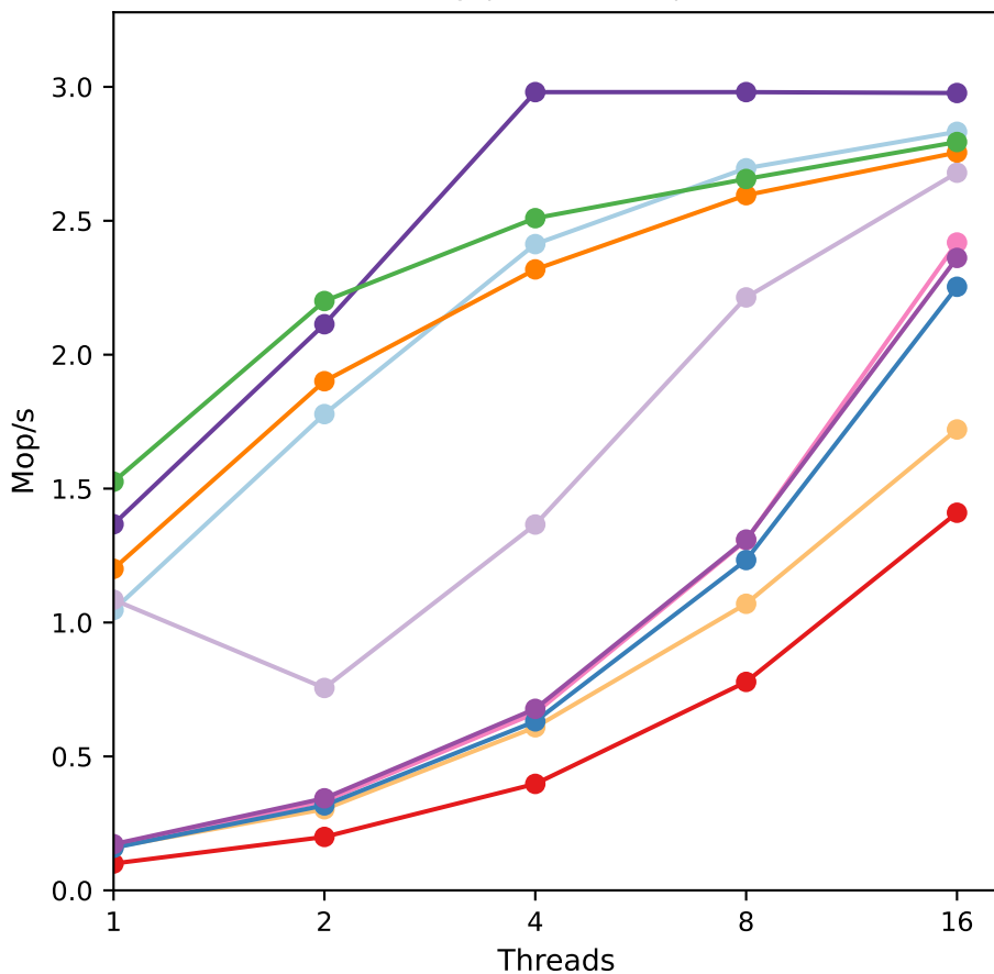
Threads vs Throughput for sm110p with 4096 size
