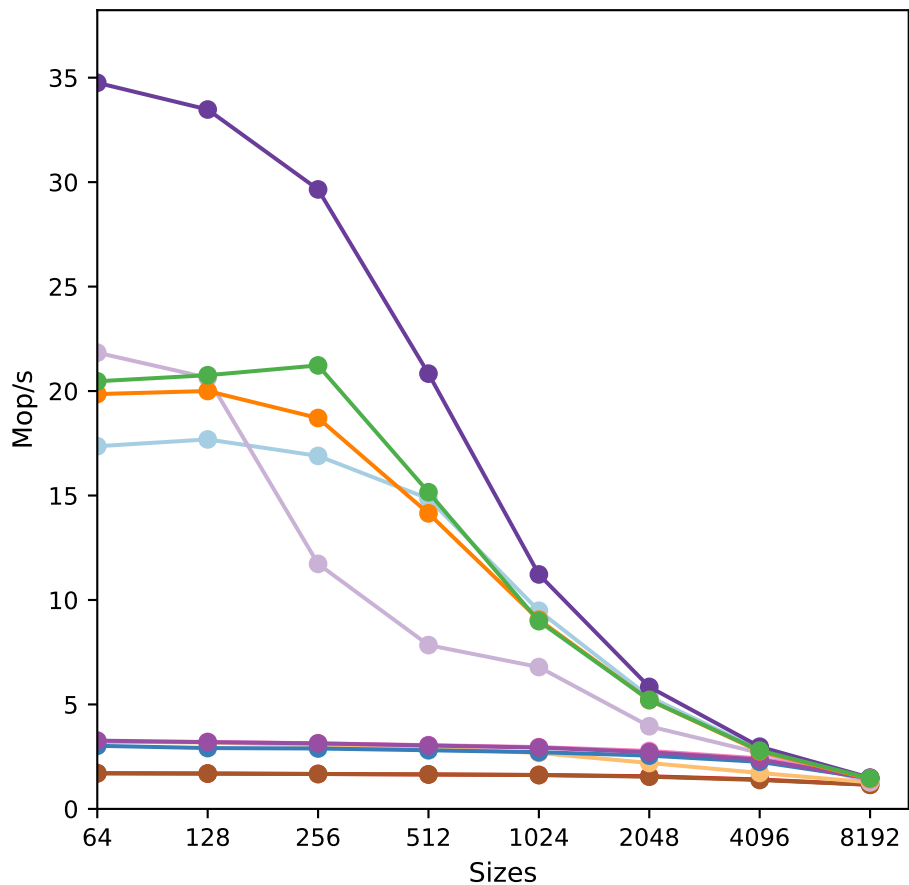
Sizes vs Throughput for sm110p with 16 threads
