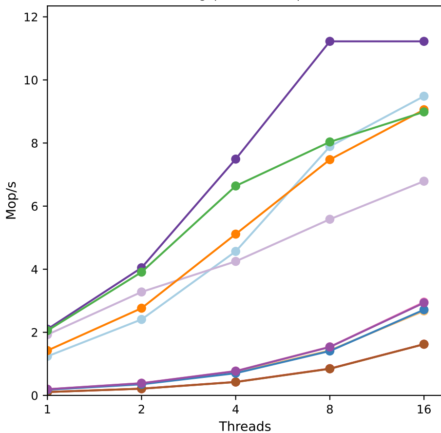
Threads vs Throughput for sm110p with 1024 size
