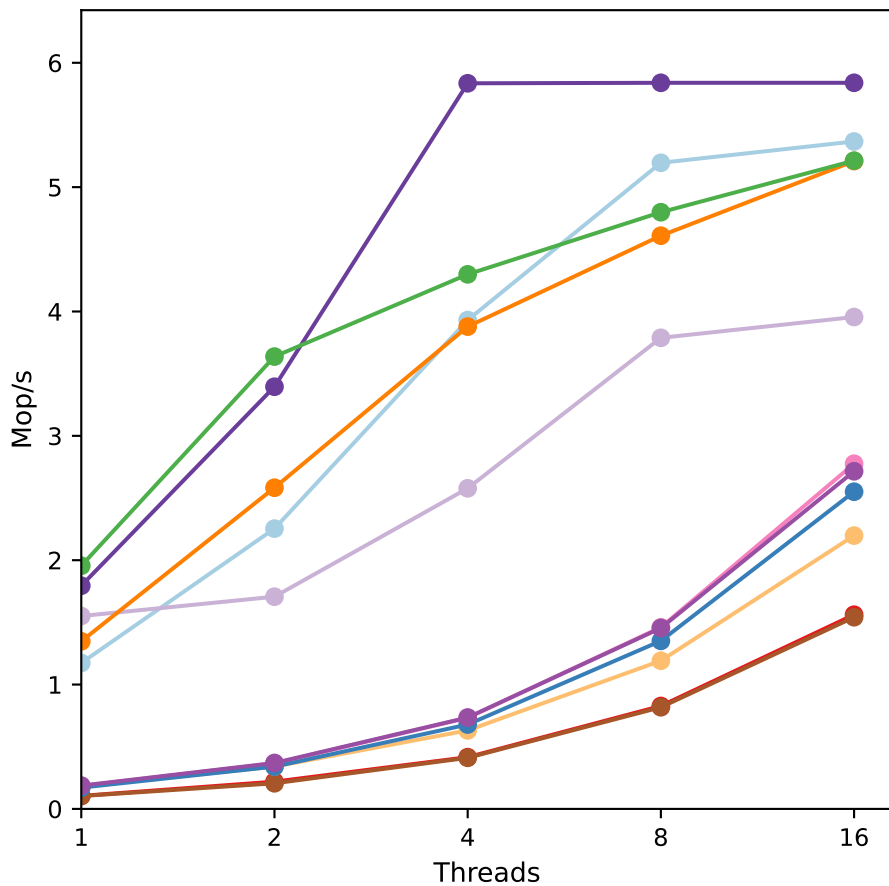
Threads vs Throughput for sm110p with 2048 size
