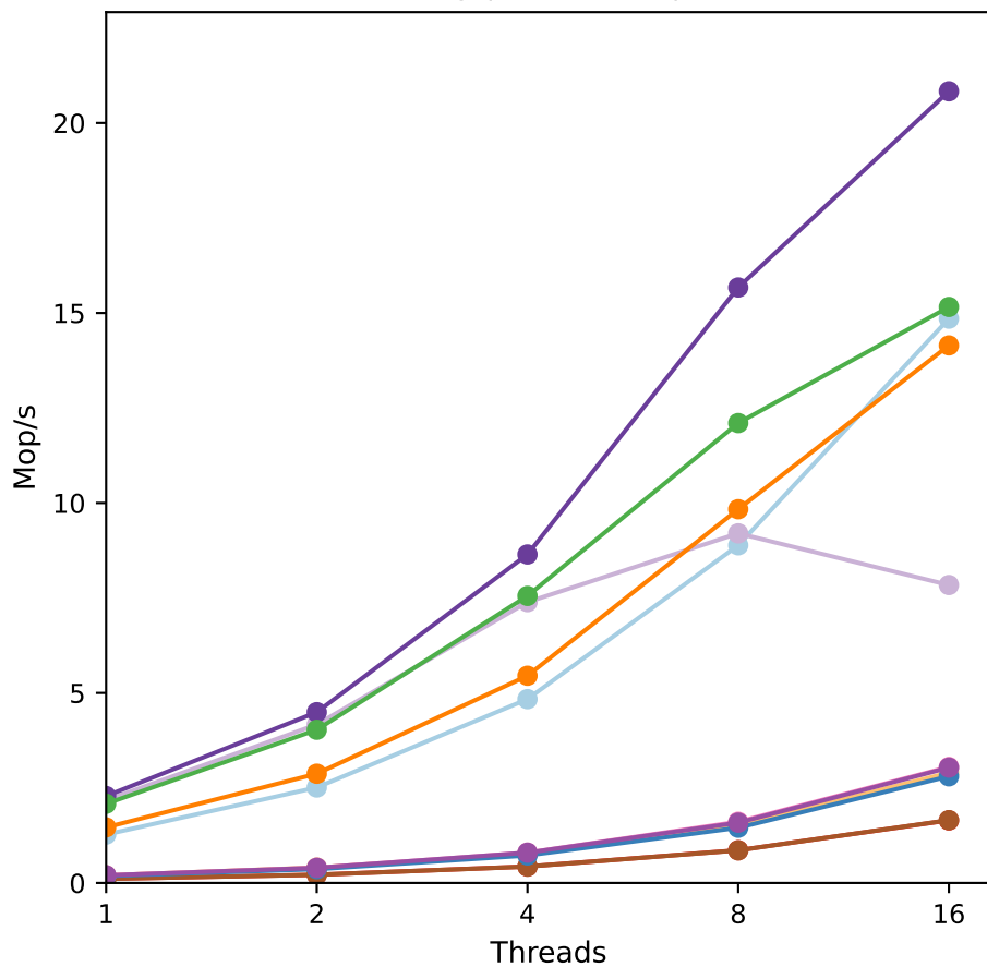
Threads vs Throughput for sm110p with 512 size
