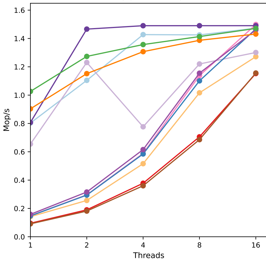
Threads vs Throughput for sm110p with 8192 size
