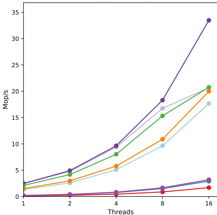
Threads vs Throughput for sm110p with 128 size
