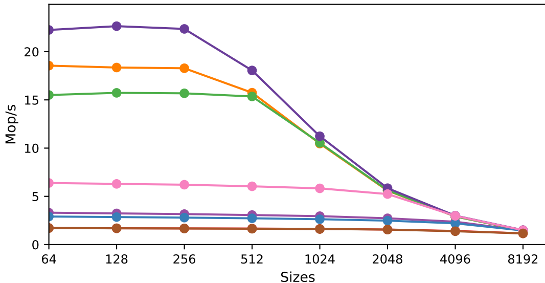
Sizes vs Throughput for sm110p with 16 threads
