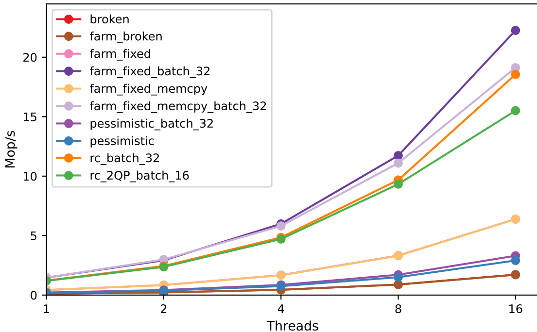
Threads vs Throughput for sm110p with 64 size
