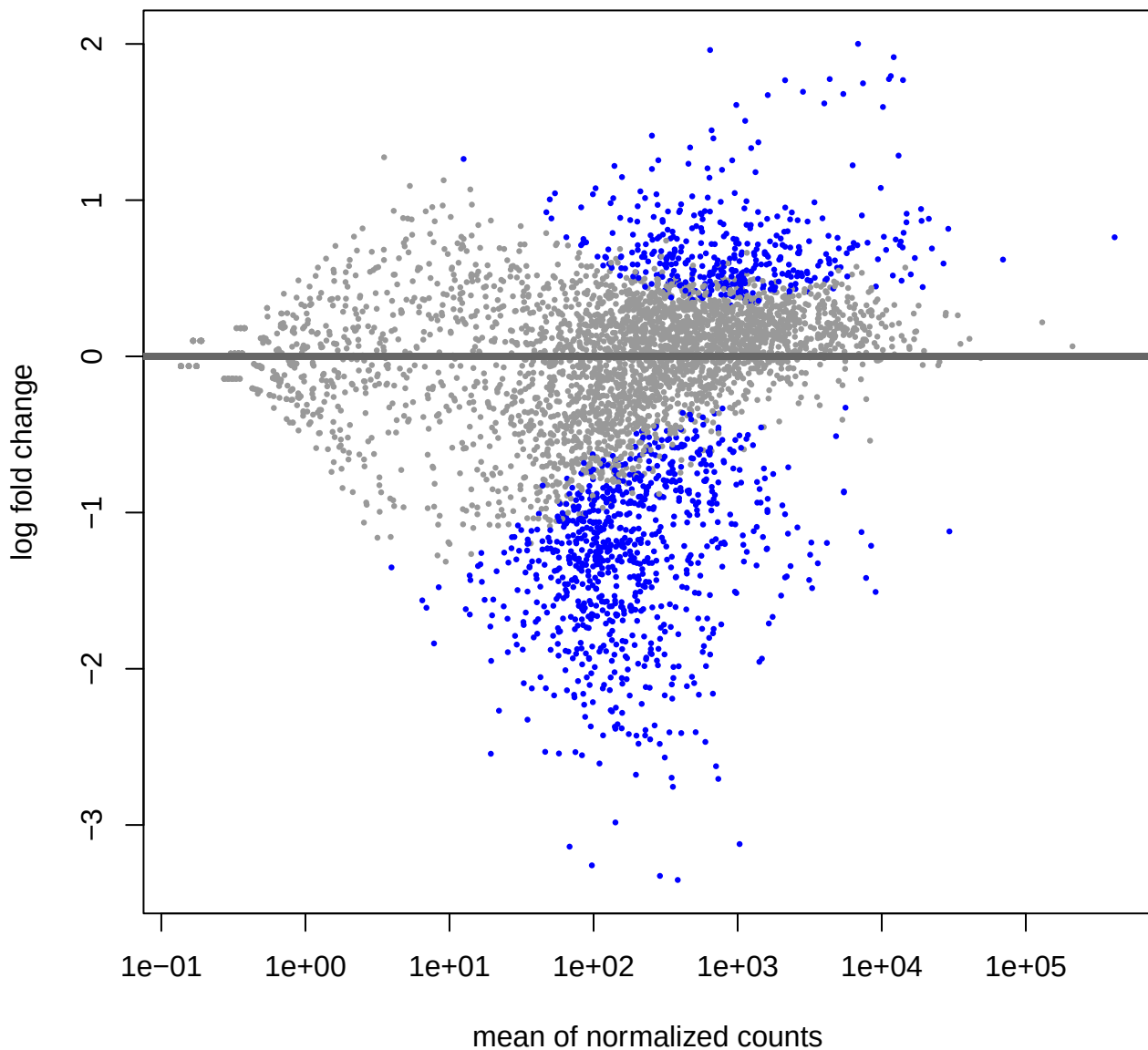
MA-plot for Condition: Wildtype vs Mutant
