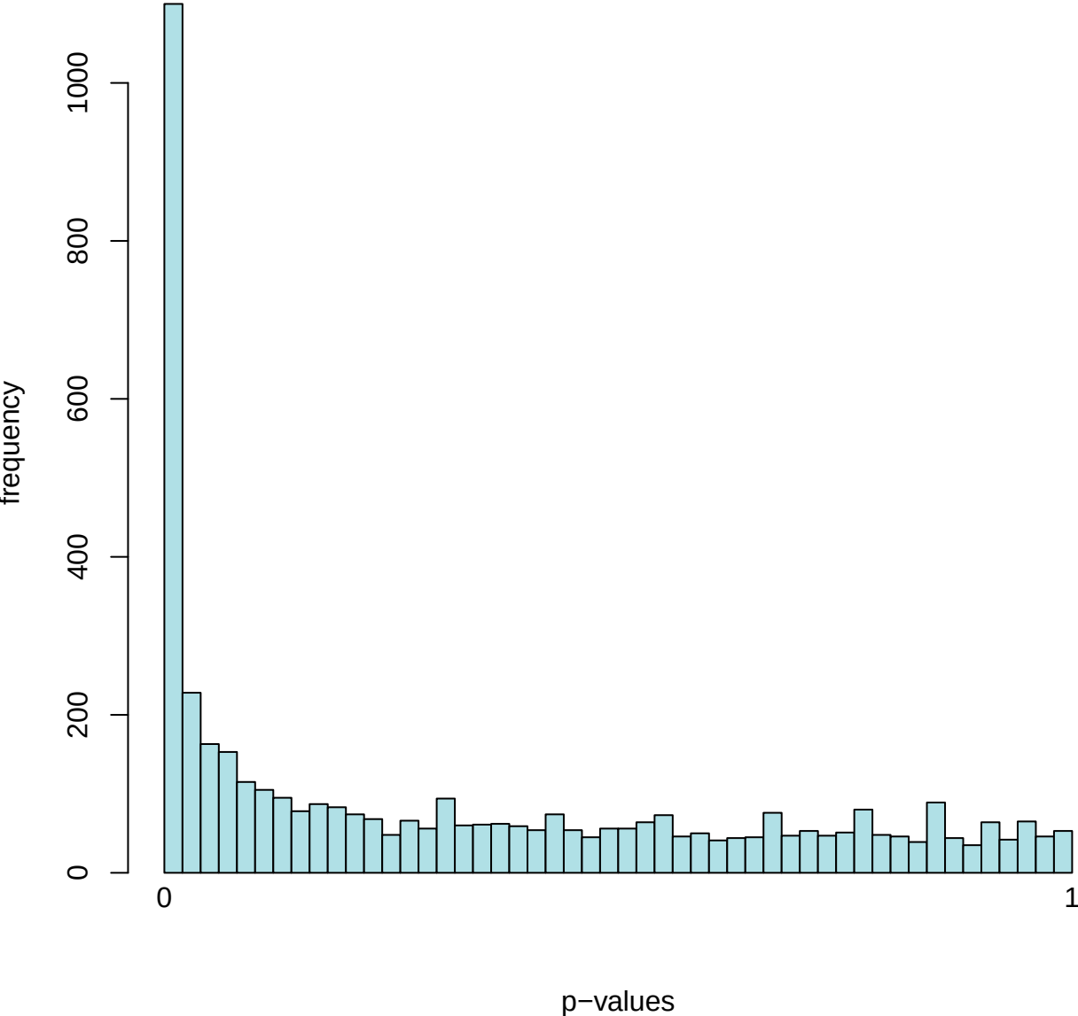
Histogram of p-values for Condition: Wildtype vs Mutant
