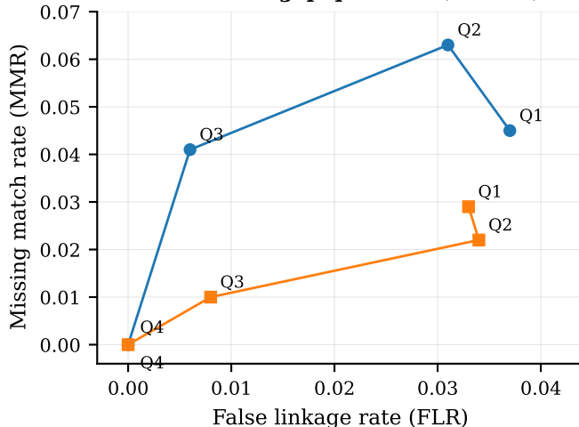
(c) DBLP-Scholar Discrimination-gap quartiles (Table 8)
