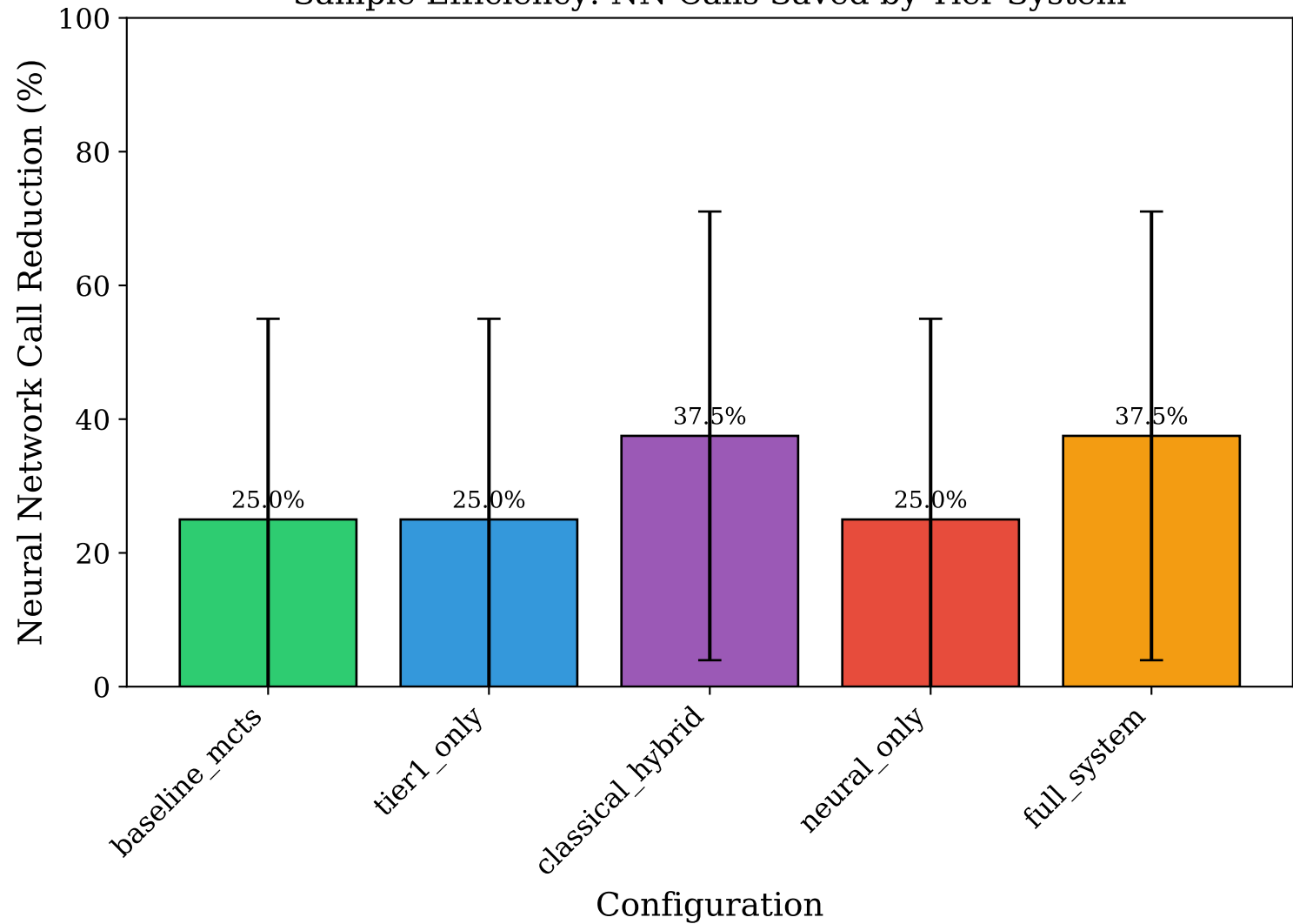
Sample Efficiency: NN Calls Saved by Tier System
