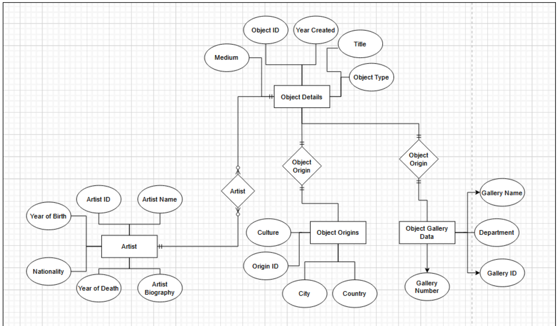
Diagram 1: Entity-Relationship Diagram
