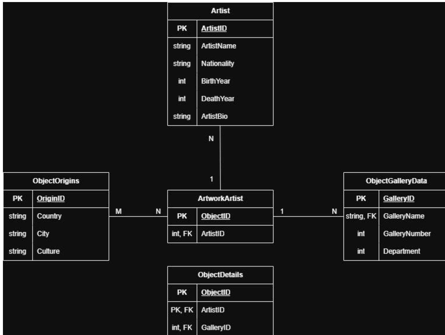
Diagram 3: Relational Schema:
