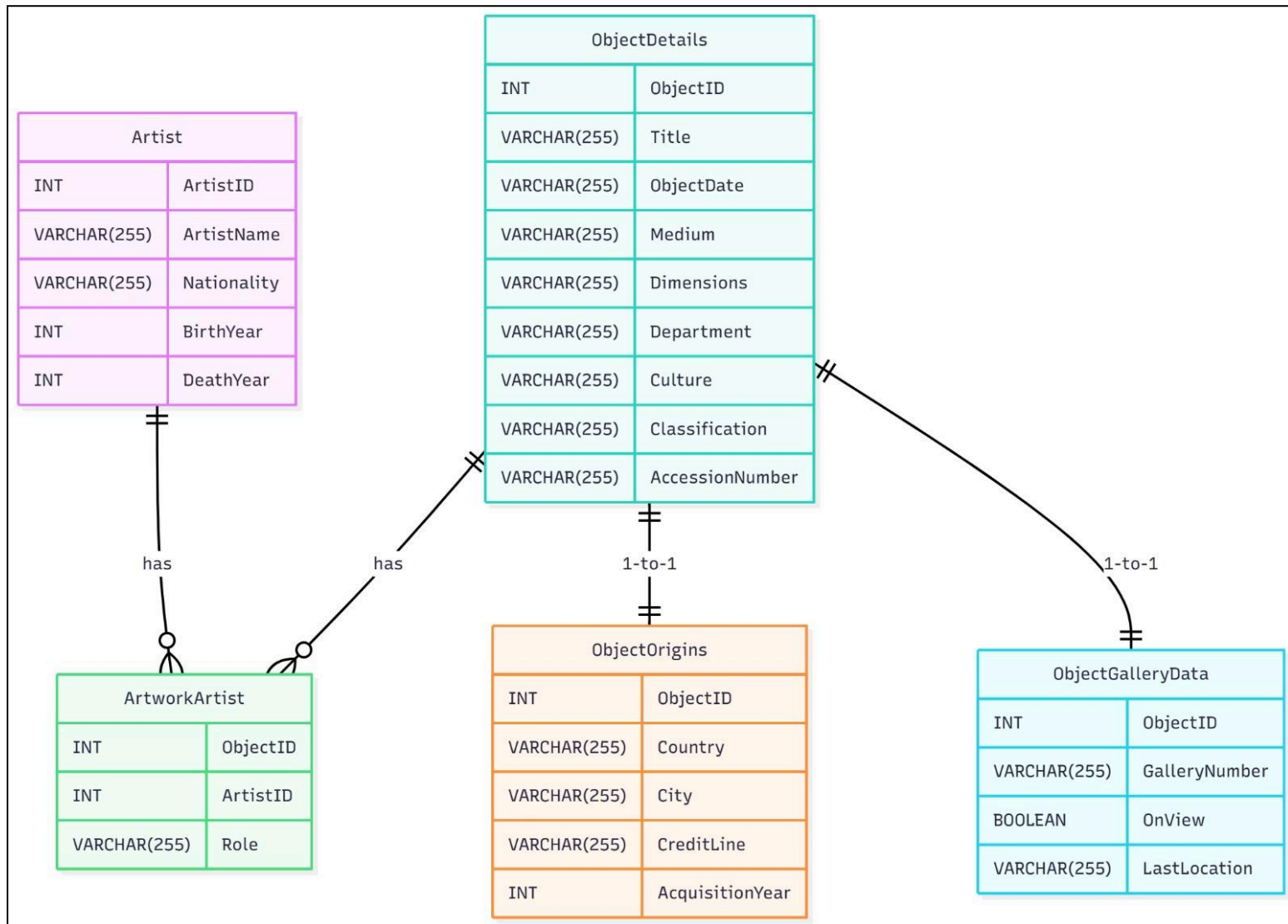
Diagram 2: Architecture Diagram:
