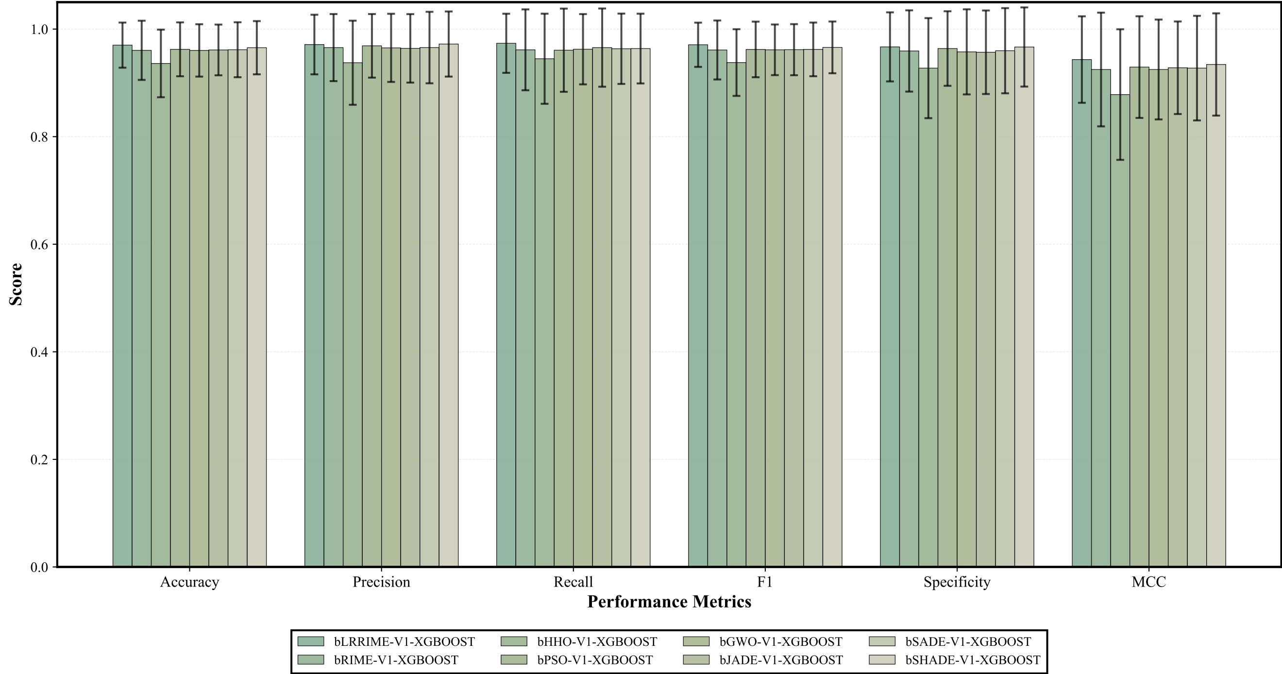
Algorithm Performance Comparison (Mean \pm Std)
