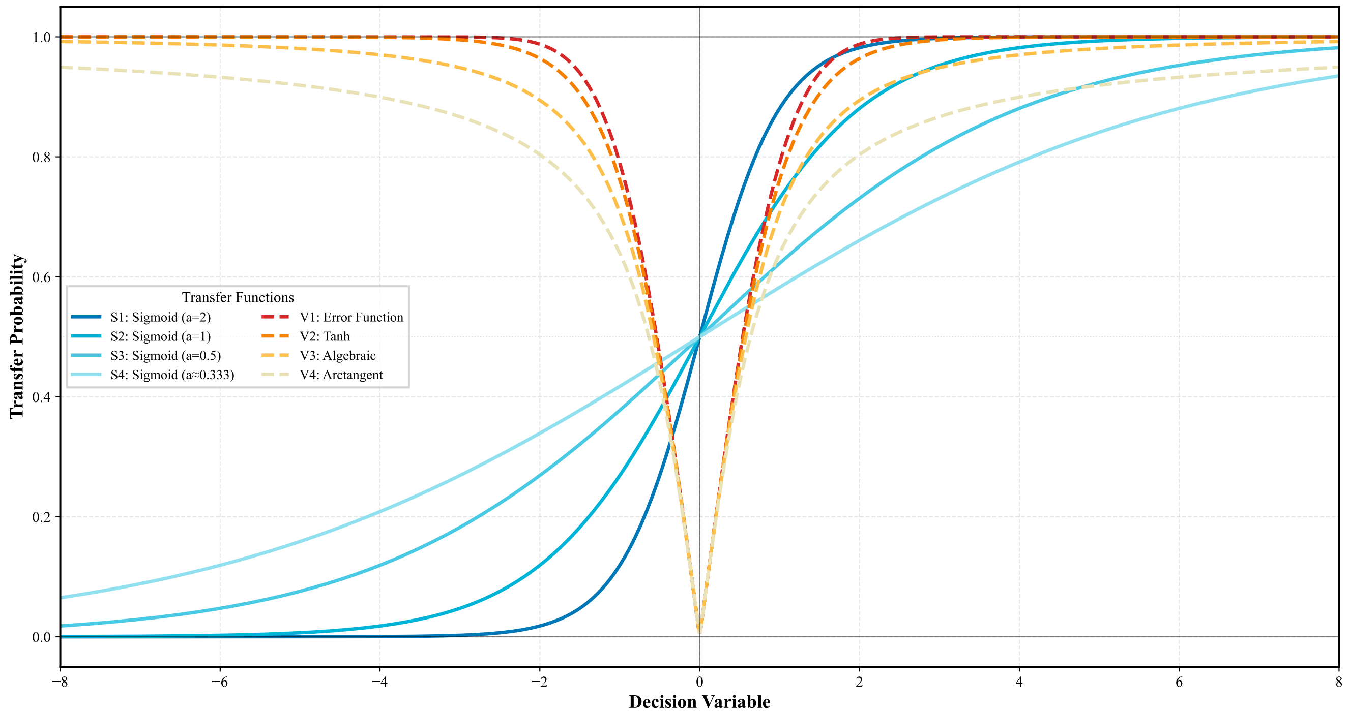
Binary Transfer Functions for Metaheuristic Optimization
