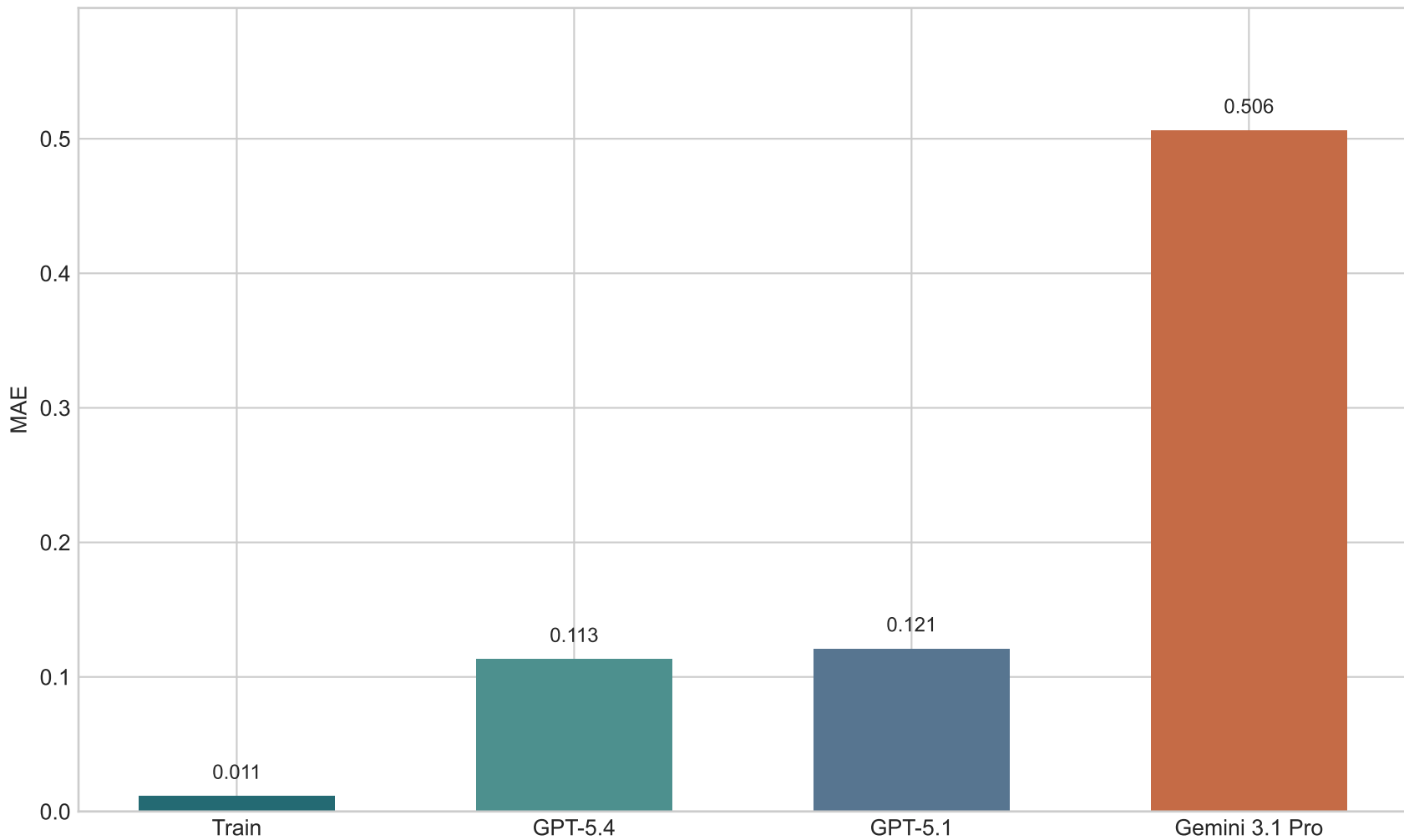
Predictor Transfer Gap: In-Distribution vs Frontier OOD
