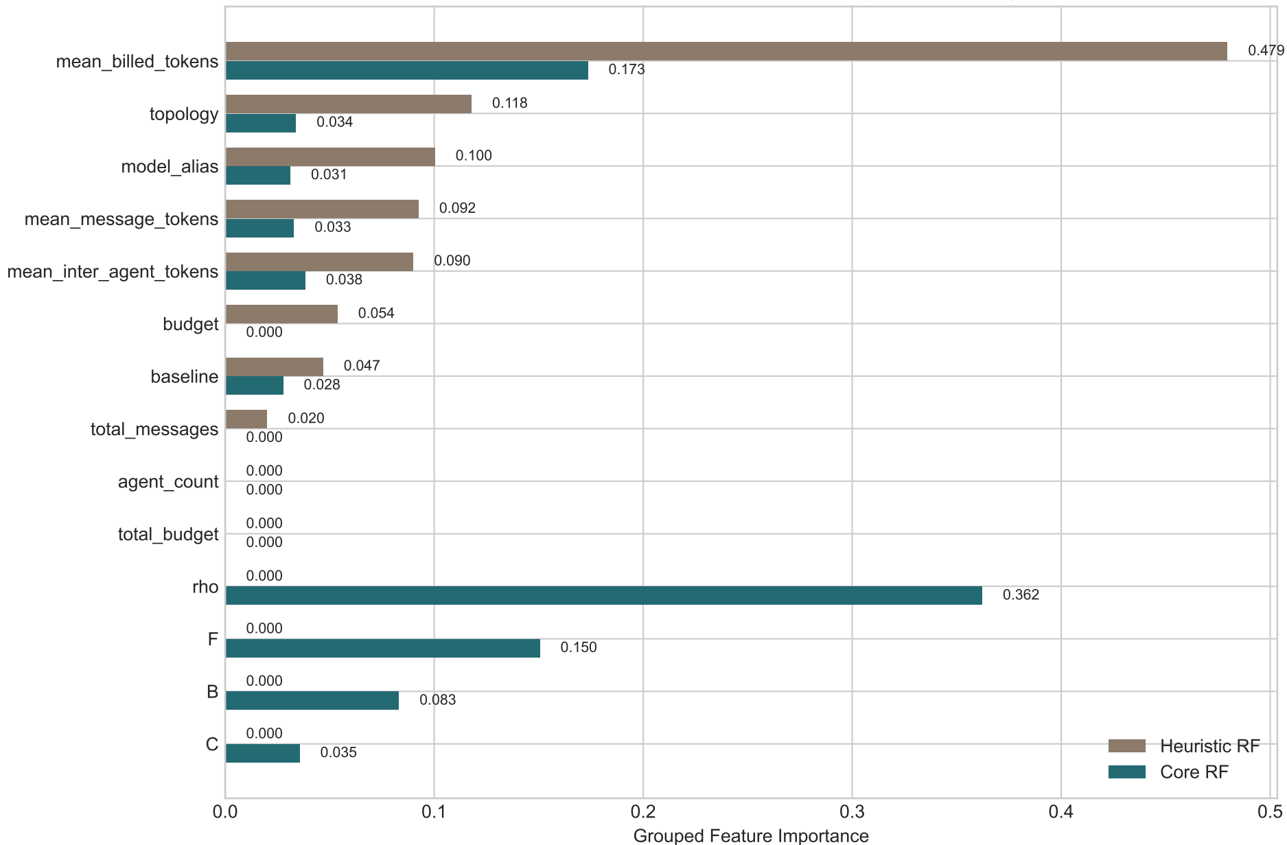
Feature Importance: Heuristic vs Core (`help_vs_rest`)
