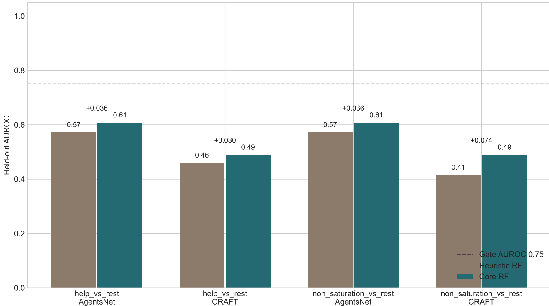
Held-out Family AUROC: Heuristic vs Core
