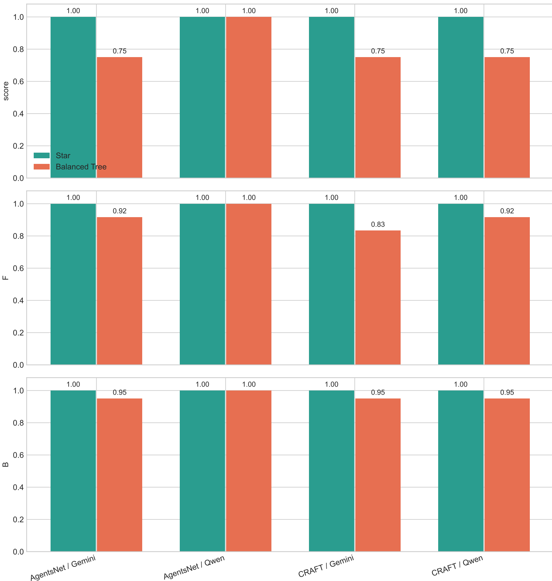
Topology Penalty: Star vs Balanced Tree (`MA-FT`, budget 96)
