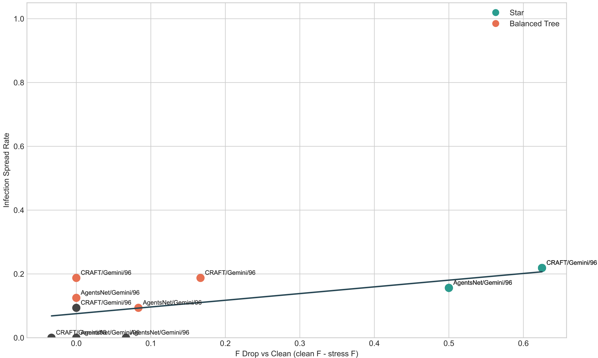
Natural Quarantine Tradeoff: Useful Fact Loss vs Viral Spread
