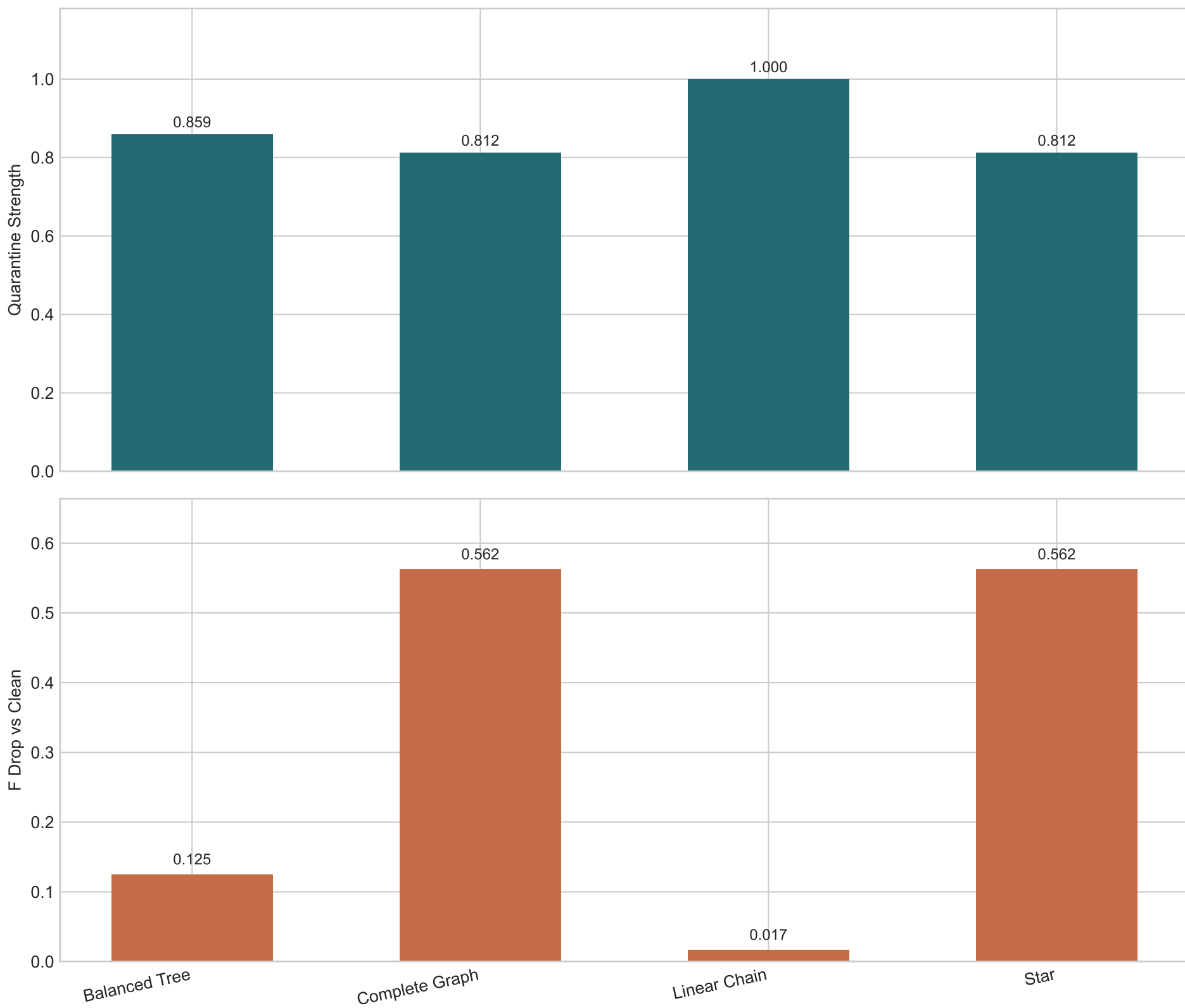
Leaf Attack: Quarantine Strength vs F Drop Across Topologies (`MA-FT`, Gemini, budget 96)
