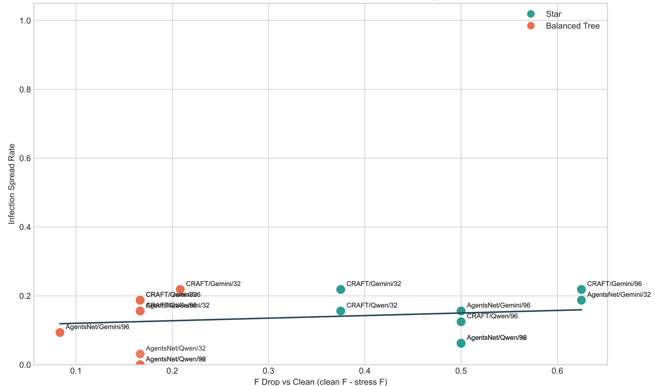
Natural Quarantine Tradeoff: Useful Fact Loss vs Viral Spread
