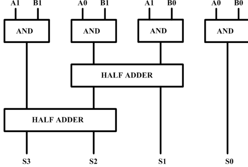
Fig. 2. Designing of 2-bit Vedic multiplier (2-bit VM) using two Half adders(HA)
