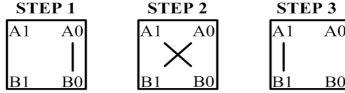
Fig. 1. Implementation of 2-bit Vedic multiplication process using Urdhva Triyakbhyam Principle
