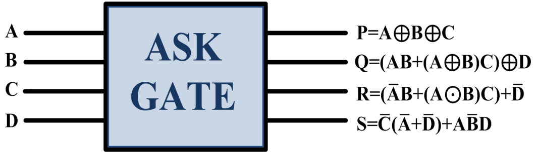
Fig. 3. Proposed reversible ASK Gate
