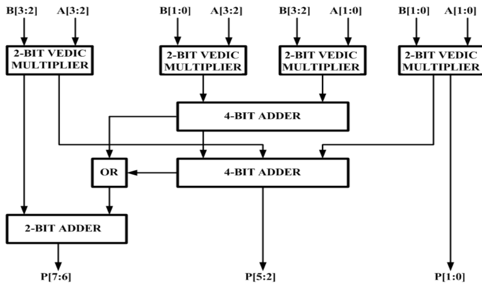
Fig. 5. Implementation of 4-bit Vedic multiplier(VM) using proposed ASK Gate
