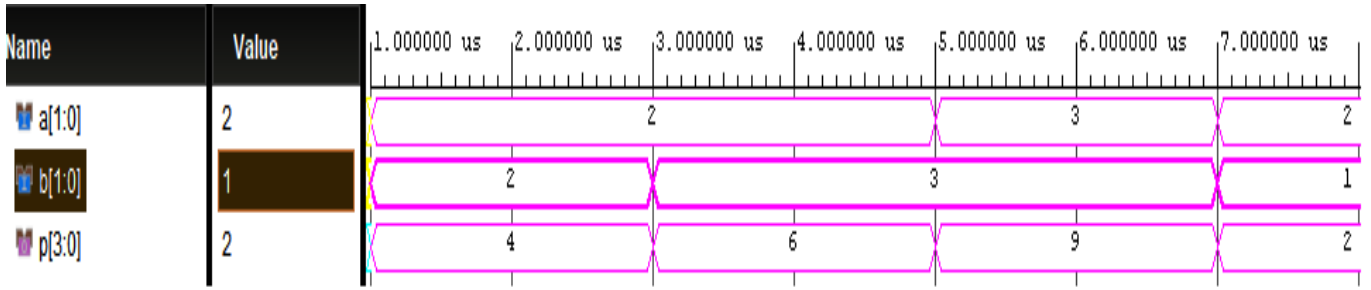
Fig. 7. Simulation output of 2-bit Vedic multiplier
