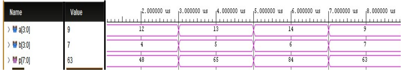
Fig. 8. Simulation output of 4-bit Vedic multiplier using proposed ASK Gate
