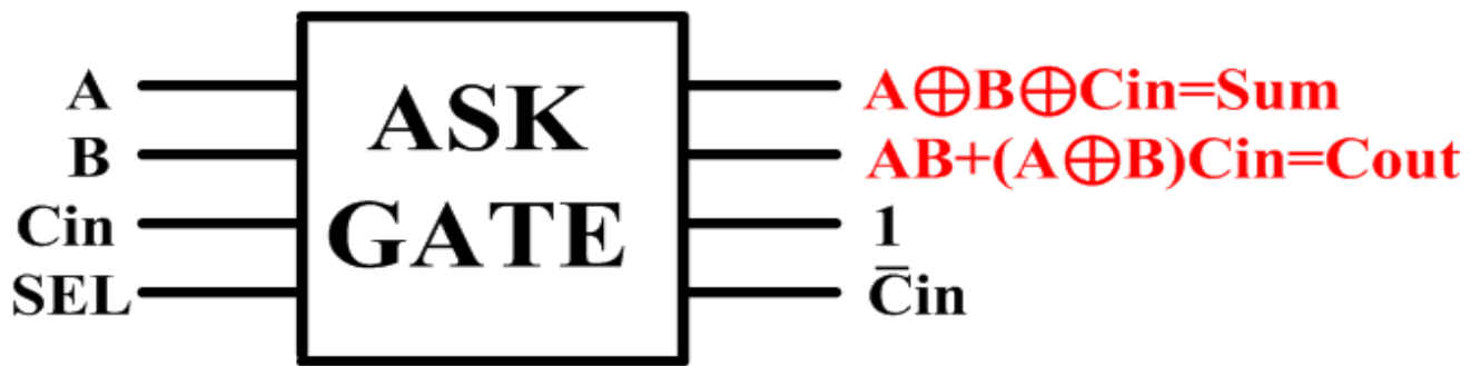
Fig. 4. Implementation of Full adder using proposed ASK Gate
