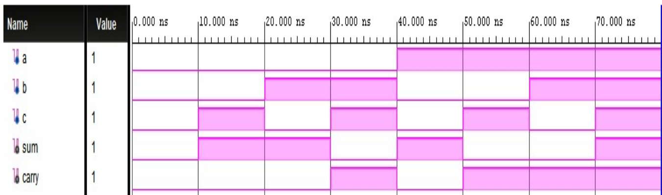
Fig. 6. Simulation output of full adder using proposed ASK Gate
