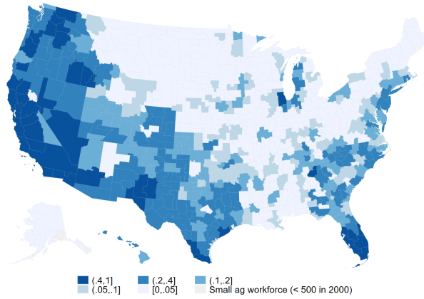
(a) PANCAL share of ag laborers, 2000
