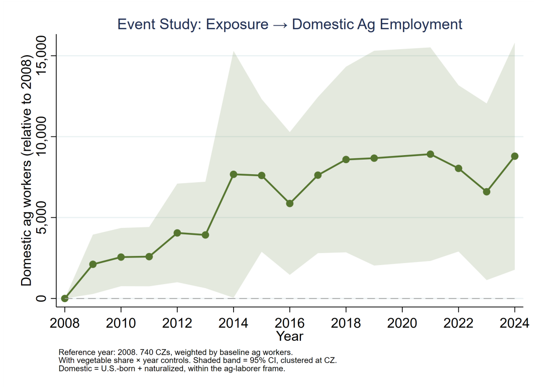
FIGURE 5. Event Study of Domestic Agricultural Employment on Baseline PANCAL Exposure
