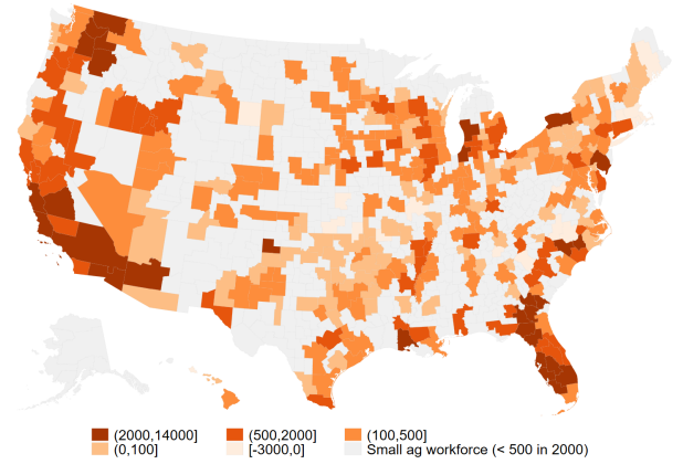
(b) Change in H-2A workers, 2022-2024 vs 2008-2010
