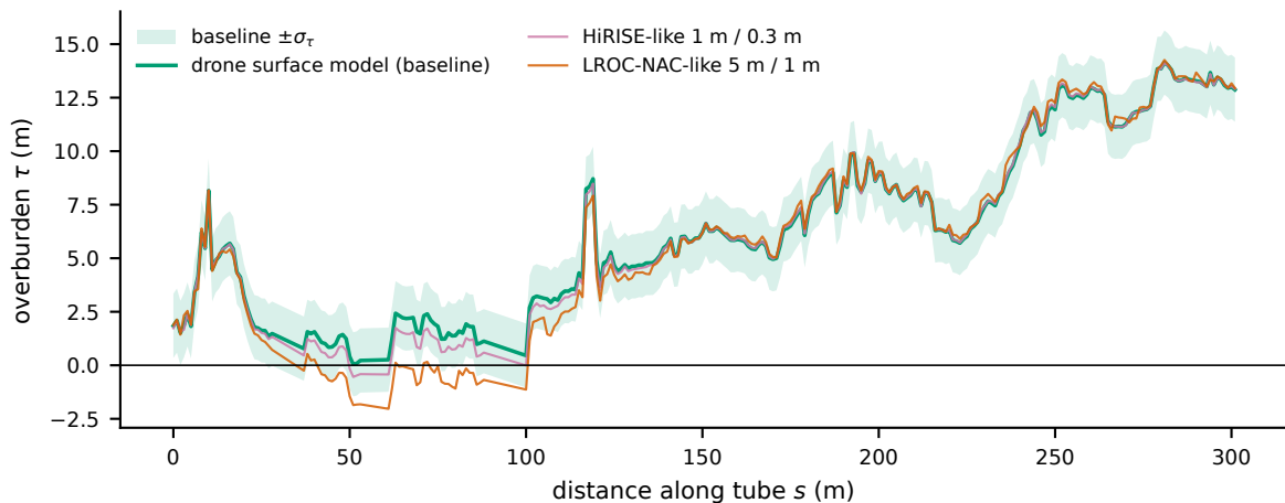
c The same profile measured against surfaces of orbital DTM quality (single realisations)
