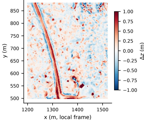
a Photogrammetric surface minus ArcticDEM (constant datum removed)
