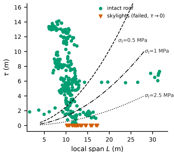
c Thickness against span, with the clamped-strip stability limit
