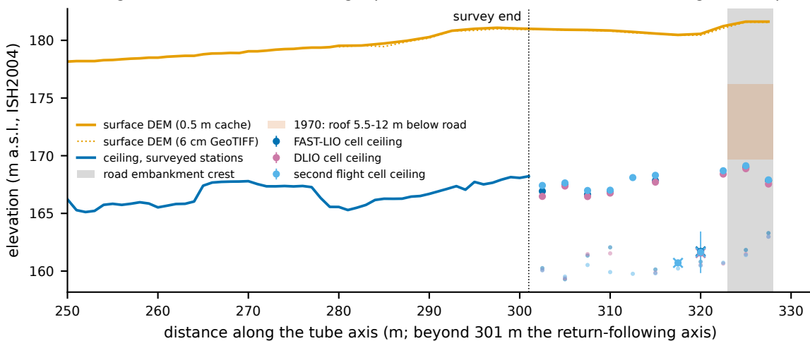
a Long section at the road crossing; open circles: < 30 returns; crosses: ceiling not sampled
