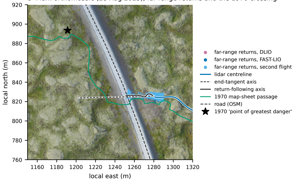
b Plan: orthomosaic (28 Aug 2025), far-range returns and the 1970 crossing
