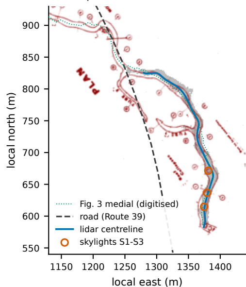
a Ellis 1971 Fig. 3 over the lidar shell (shape fit, RMS 3.7 m)
