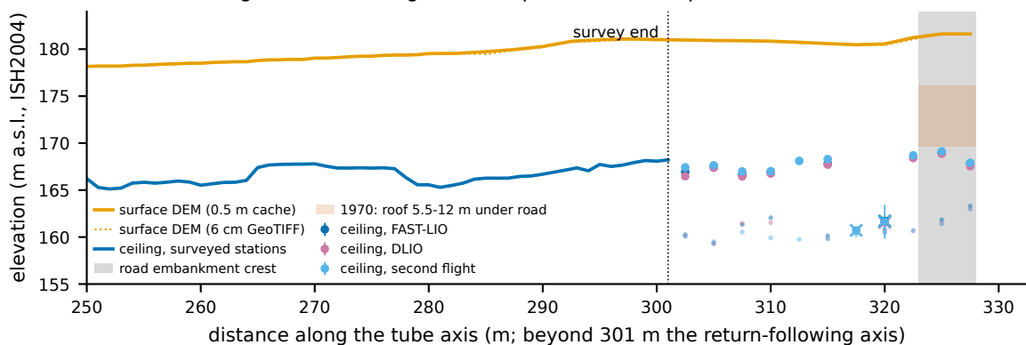
e Road crossing: surface, ceiling and floor per 2.5 m cell (open circles: < 30 returns; crosses: ceiling not sampled)
