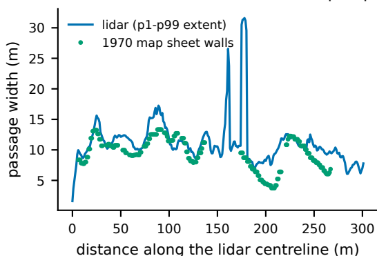
d Width: 1970/lidar median 0.86 (p10-p90 0.55-1.03)
