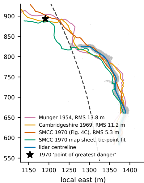
b Older plans on the same frame (medial lines)
