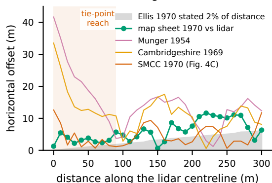
c 1970 traverses against the lidar centreline
