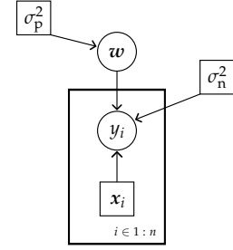
Figure 2.3: Directed graphical model of Bayesian linear regression in plate notation.
