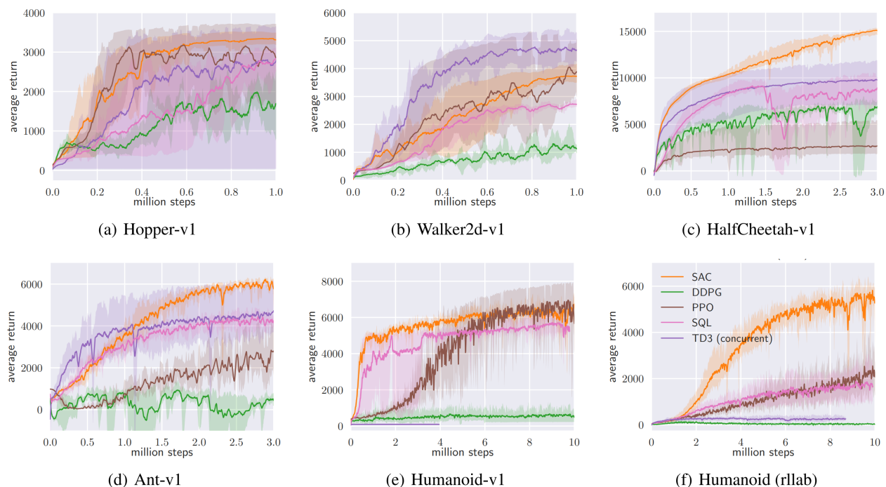
Figure 12.4: Comparison of training curves of a selection of on-policy and off-policy policy gradient methods. Reproduced with permission from “Soft actor-critic algorithms and applications” (Haarnoja et al., 2018b).
