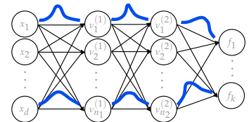
Figure 7.4: Bayesian neural networks model a distribution over the weights of a neural network.
