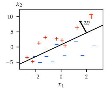
Figure 5.3: Logistic regression classifies data into two classes with a linear decision boundary.
