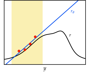
Figure 12.8: Illustration of “reward gaming”. Shown in black is the true reward r(y \mid x) for a fixed prompt x . Shown in blue is the approximation based on the feedback \mathcal{D} to the responses shown in red. The yellow region symbolizes responses y where the approximate reward can still be “trusted”.
