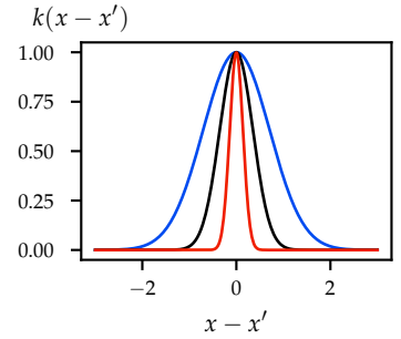
Figure 4.5: Gaussian kernel with length scales h = 1 , h = 0.5 , and h = 0.2 .
