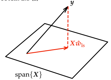
Figure 2.2: Least squares regression finds the orthogonal projection of \mathbf{y} onto \text{span}\{\mathbf{X}\} (here illustrated as the plane).
