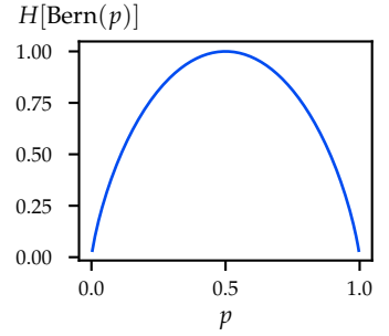
Figure 5.7: Entropy of a Bernoulli experiment with success probability p .
