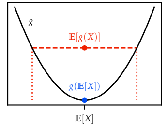
Figure 5.8: An illustration of Jensen’s inequality. Due to the convexity of g , we have that g evaluated at \mathbb{E}[X] will always be below the average of evaluations of g .
