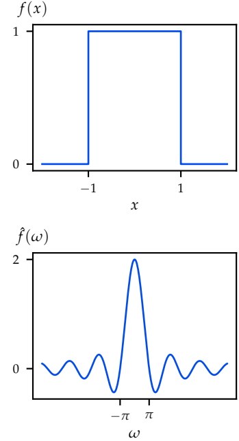
Figure 4.12: The Fourier transform of a rectangular pulse,
