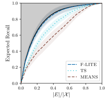
Figure 9.10: Menet et al. (2025) show in an experiment that selecting E \subseteq \mathcal{X} according to the estimates of probability of maximality from LITE (here called F-LITE) is near-optimal. Intuitive heuristics such as Thompson sampling (TS) or selecting points with the highest posterior mean (MEANS) perform worse.
