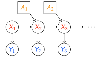
Figure 10.4: Directed graphical model of a partially observable Markov decision process with hidden states X_t , observables Y_t , and actions A_t .
