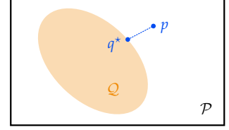
Figure 5.4: An illustration of variational inference in the space of distributions \mathcal{P} . The variational distribution q^* \in \mathcal{Q} is the optimal approximation of the true posterior p .
