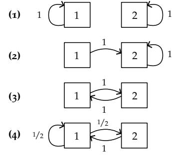
Figure 6.2: Transition graphs of Markov chains: (1) is not ergodic as its transition diagram is not strongly connected; (2) is not ergodic for the same reason; (3) is irreducible but periodic and therefore not ergodic; (4) is ergodic with stationary distribution \pi(1) = 2/3, \pi(2) = 1/3 .
