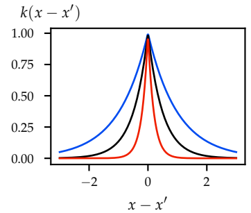
Figure 4.6: Laplace kernel with length scales h = 1 , h = 0.5 , and h = 0.2 .
