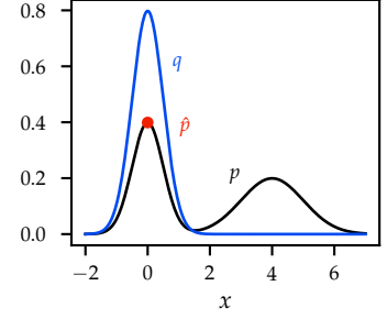
Figure 5.1: The Laplace approximation q greedily selects the mode of the true posterior distribution p and matches the curvature around the mode \hat{\mu} . As shown here, the Laplace approximation can be extremely overconfident when p is not approximately Gaussian.
