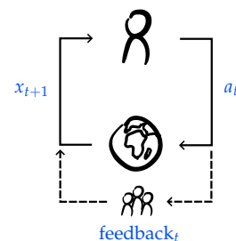
Figure 12.5: We generalize the perspective of reinforcement learning from Figure 11.1 by allowing the feedback to come from either the environment or an evaluation by other agents (e.g., humans), and by allowing the feedback to come in other forms than a numerical reward.
