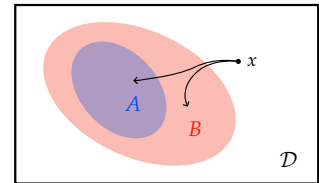
Figure 8.3: Monotone submodularity. The effect of “adding” x to the smaller set A is larger than the effect of adding x to the larger set B .
