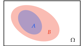
Figure 1.2: Conditioning an event A on another event B can be understood as replacing the universe of all possible outcomes \Omega by the observed outcomes B . Then, the conditional probability is simply expressing the likelihood of A given that B occurred.
