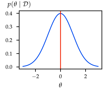
Figure 1.8: A the MLE/MAP are point estimates at the mode \hat{\theta} of the posterior distribution p(\theta \mid \mathcal{D}) .
