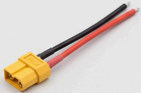
Male XT60 Connector w/Pigtail
