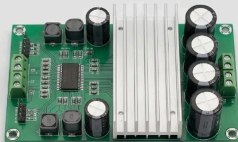
TDA7498E 2 x 160W dual channel amp board
