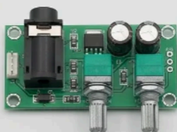
Karaoke microphone amp module
