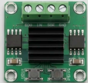
2 x 15W stereo digital power amplifier
