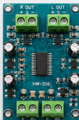
15W + 15W Stereo Amplifier Board
