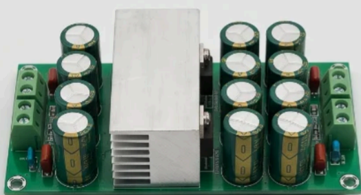
High power digital amp board
