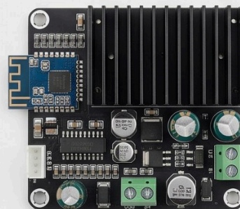
2.1CH App Control BT5.0
