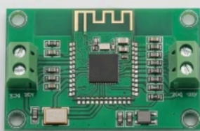
Wireless digital audio receiver amp board
