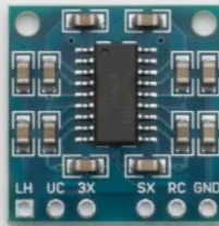
Bare PAM8403 2 x 3W class D amplifier board
