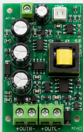
18W Audio Amplifier Board with Onboard Power Supply
