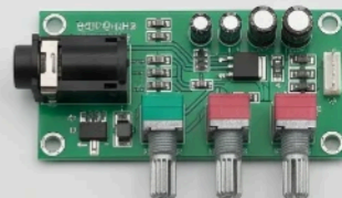
Second karaoke mic amp module
