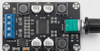
TPA3116 2x50W
