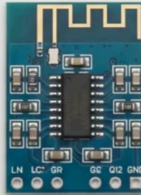
PAM8403 Bluetooth 5.0 2 x 5W module
