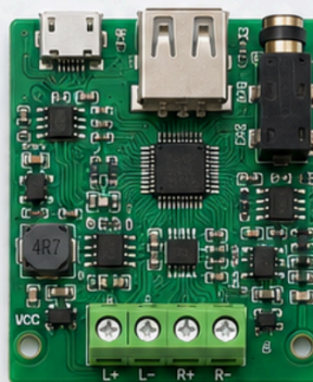
2 x 30W Amplifier Board
