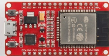
ESP32 development
