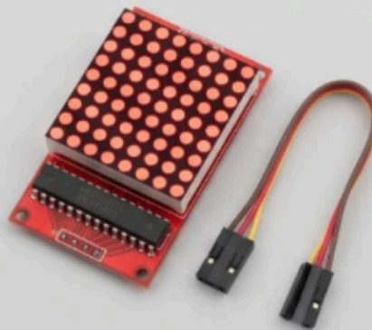
8 x 8 red LED dot matrix ribbon jumper cable
