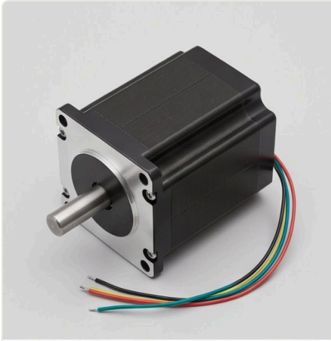
1) NEMA23 stepper motor, large square black body, thick steel shaft, four-wire lead
