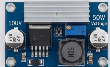
50W Adjustable Buck
