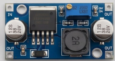
Step Down 3A Adjustable
