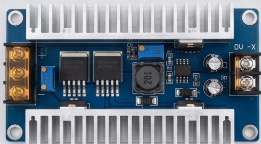
300W 20A Step Down
