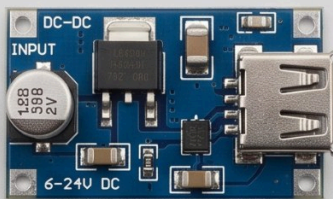
USB Step Down Charger
