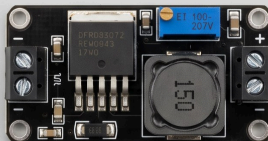
150-400W Boost Converter
