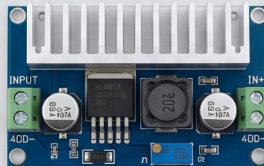
300W 10A Step Down
