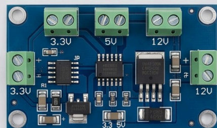
Multi Output Power Module
