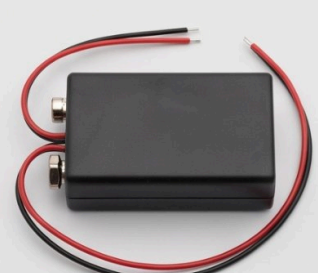
4 x 18650 Cell Holder with Wires
