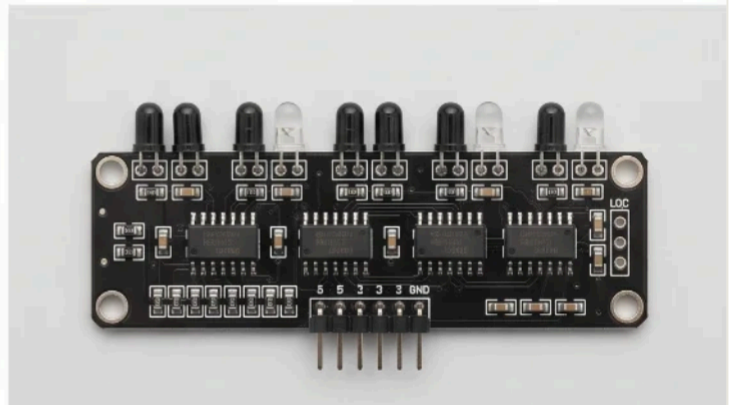
BFD-1000 5-channel infrared tracking module
