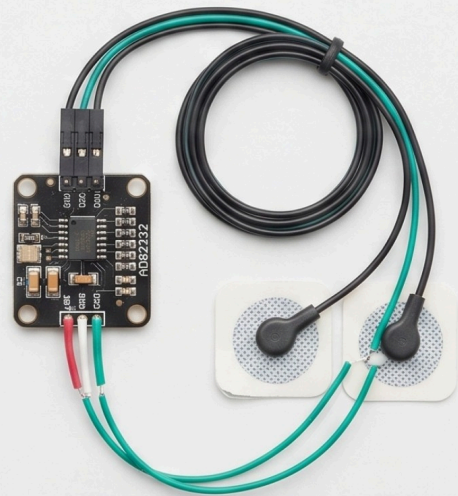
AD8232 ECG Kit
