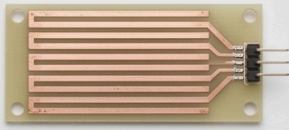
Rain Level Sensor Board
