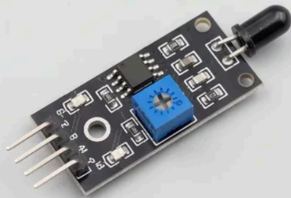
4-pin flame sensor module
