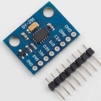
GY-291 Accelerometer
