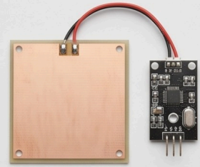
Raindrop Sensor + Plate
