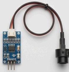
Turbidity Sensor
