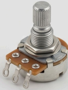
16mm Tone Knurled 15mm
