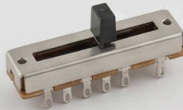
45mm Slide SC4582GG
