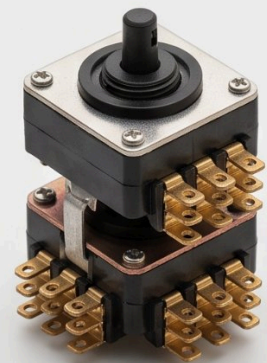
Selector Switch 6+6 Way
