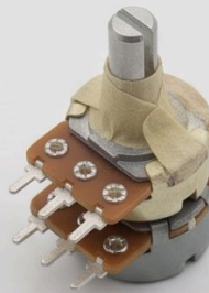
16mm Tone Dual With Tape
