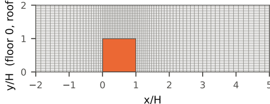
(c') Centre-plane mesh near the cube ( z = 0 )
