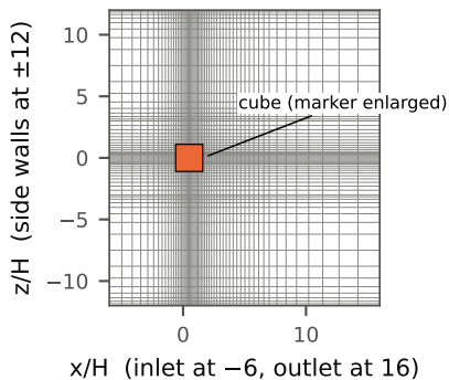
(c) Cube: floor mesh, plan view (every 2nd line)
